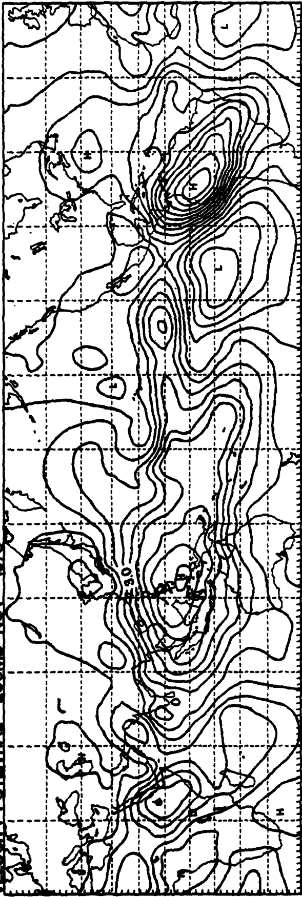
VELOCITY POTENTIAL 200MB NOV 1978
